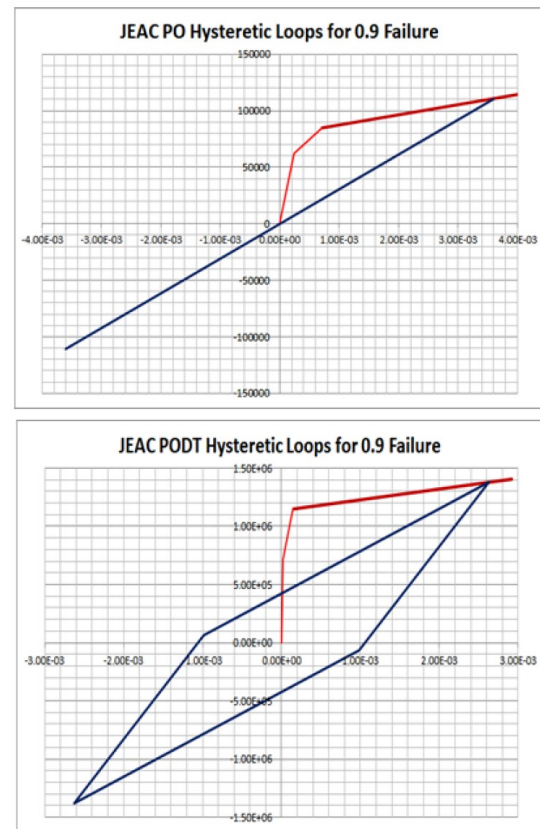
Figure 9 Stable Hysteretic Loops for JEAC PO for Shear and PODT for Bending
