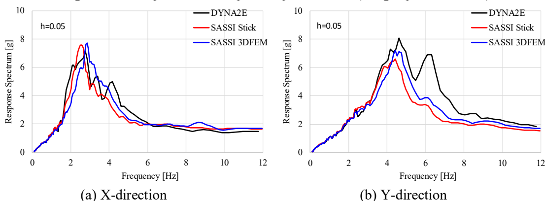
(a) X-direction (b) Y-direction Figure 17 Comparison of Response Spectra at RF (0.6 g Input Nonlinear)
