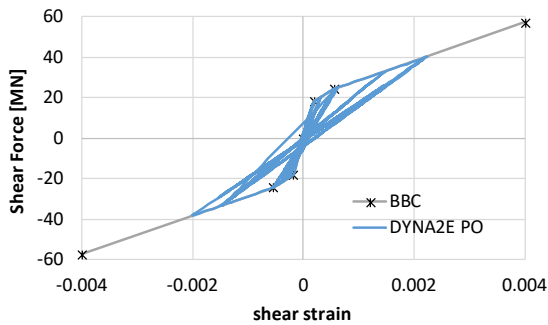
Figure 10 Example of PO Hysteresis Loop
