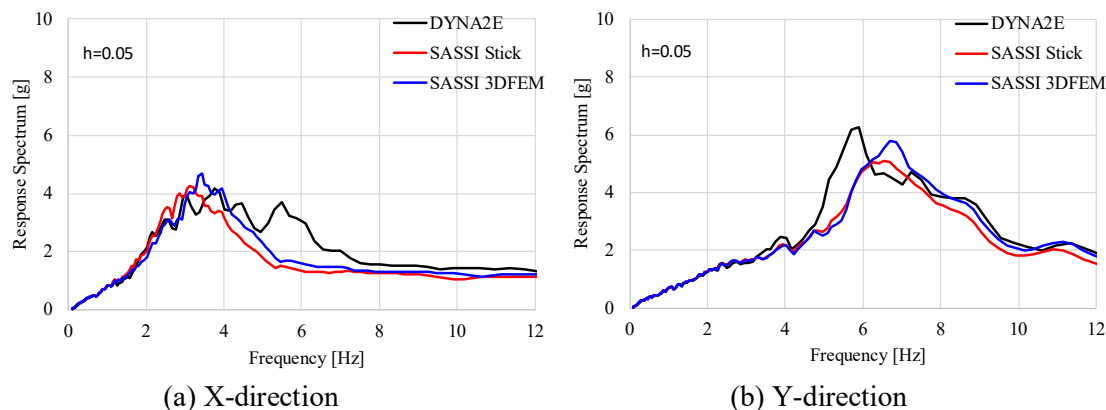
(a) X-direction (b) Y-direction Figure 16 Comparison of Response Spectra at RF (0.4 g Input Nonlinear)
