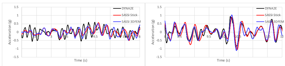
(a) Early time-frame (2-6 sec) (b) Maximum response time-frame (8-12 sec) Figure 18 Comparison of Acceleration Time History at RF (0.4 g Input, X-dir.)
