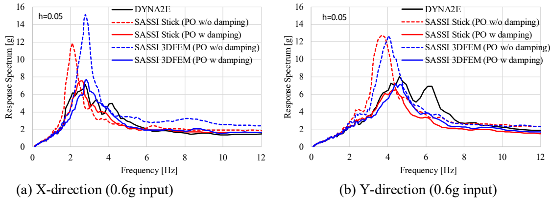
Figure 12 Comparison of Response Spectra at RF between PO model Without and With Damping
